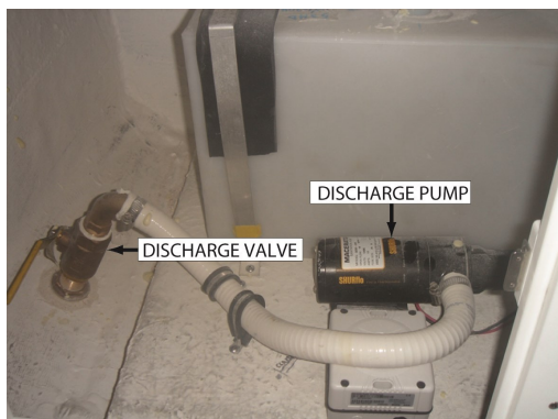
Gamefish 30 toilet pump and valve layout
