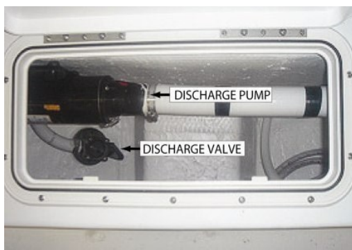
Gamefish 25/27 & Ultra 255 SE, Ultra 275 SE toilet pump and valve layout
